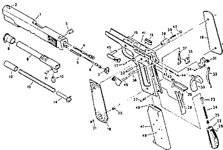
FIGURE 12 – COLT® GOVERNMENT MODEL® MKIV™/Series 70 MODEL O1970A1™ PARTS ILLUSTRATION
