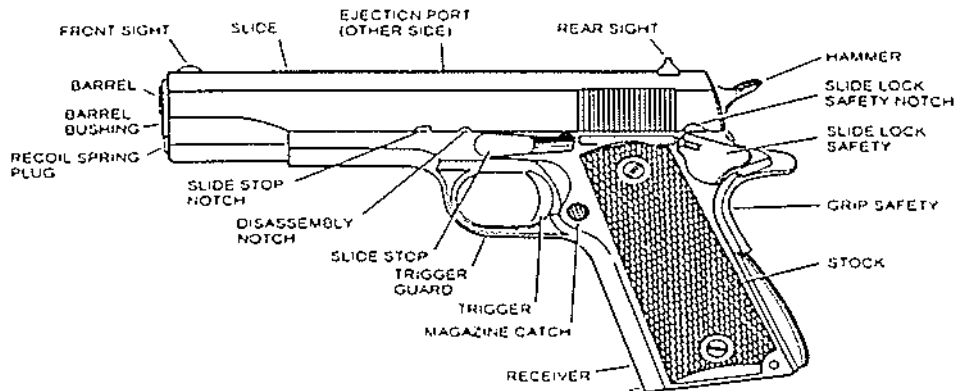
FIGURE 1 – COLT® GOVERNMENT MODEL® MKIV™/Series 70 MODEL O1970A1™
